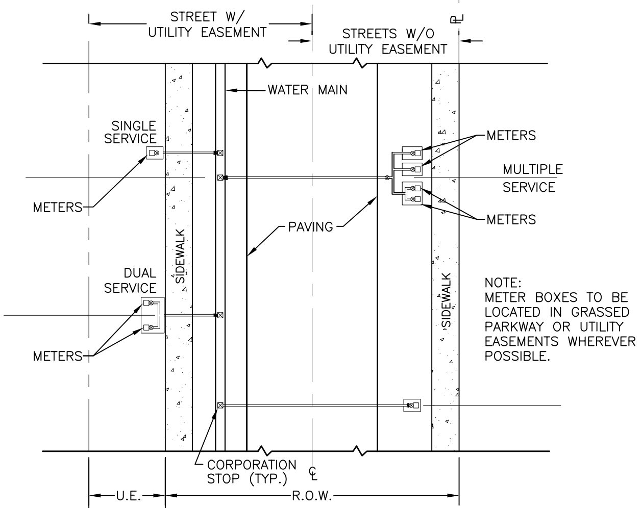
PLAN VIEW
